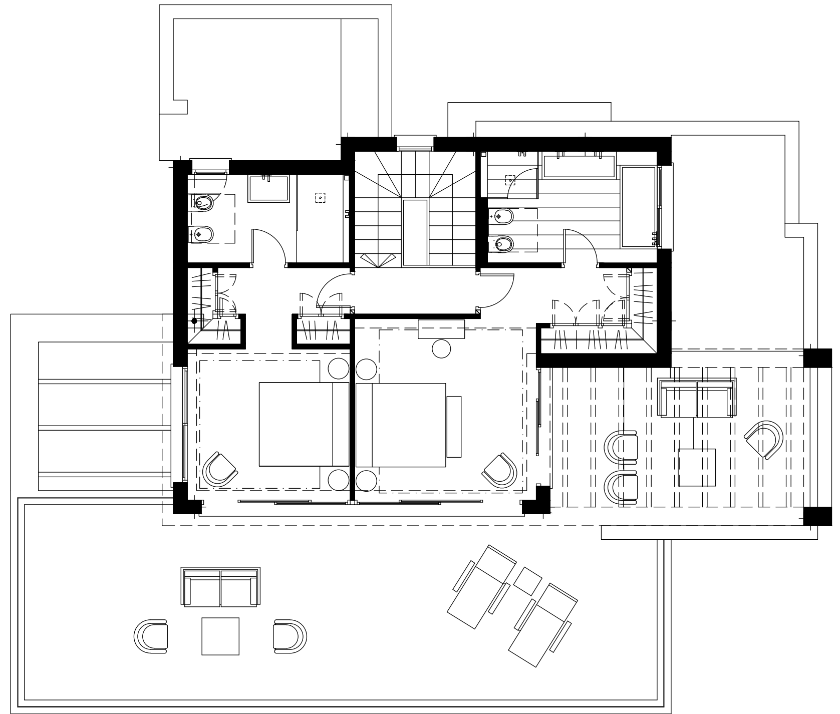
PINO 3 | FIRST FLOOR
